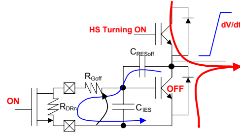
Figure 21: R Goff Sizing: Current Path When Low Side is Off and High Side Turns On
