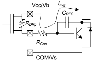
Figure 20: R Gon Sizing
