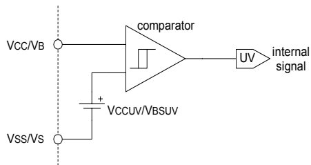
Figure 1: Undervoltage Diagram
