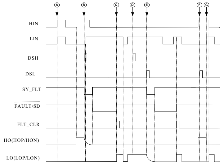
Figure 16: I/O Timing Diagram with \overline{\text{SY\_FLT}} and \overline{\text{FAULT/SD}} as Output
