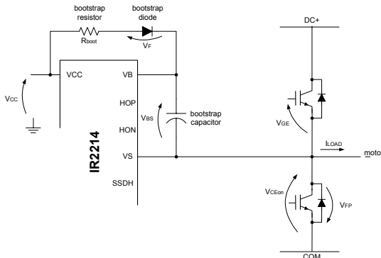
Figure 18: Bootstrap Supply Schematic
