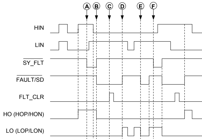
Figure 17: I/O Logic Diagram with \overline{\text{SY\_FLT}} and \overline{\text{FAULT/SD}} as Input
