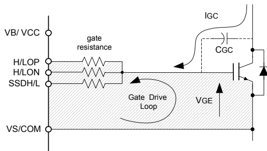
Figure 22: gate drive loop
