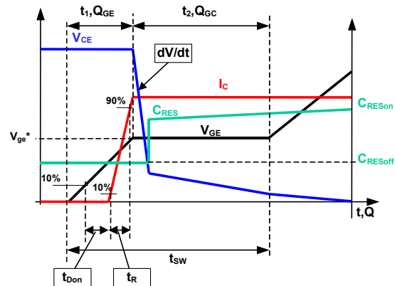
Figure 19: Nomenclature
